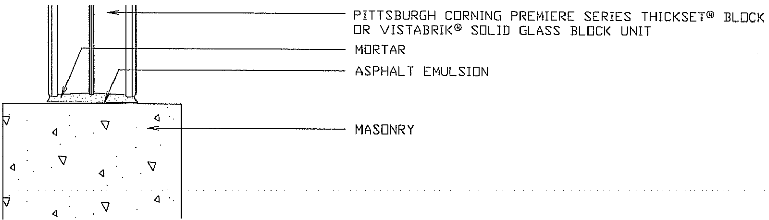
○ SILL - 90 MINUTE FIRE RATED GLASS BLOCK PANEL 1/4 FS
